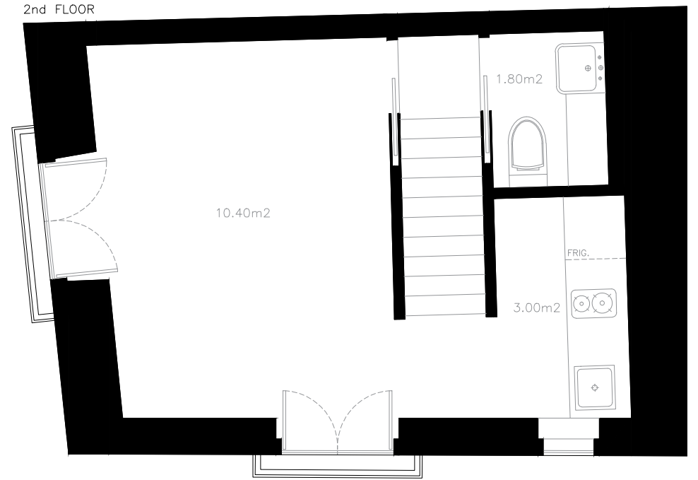
PISO 2 2nd FLOOR
