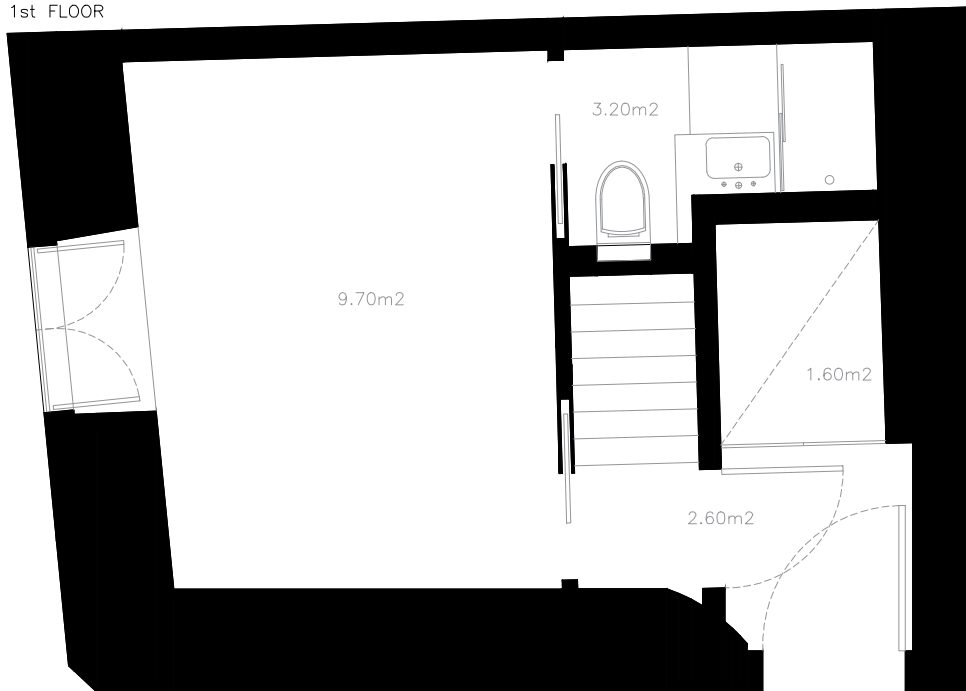
PISO 1 1st FLOOR
