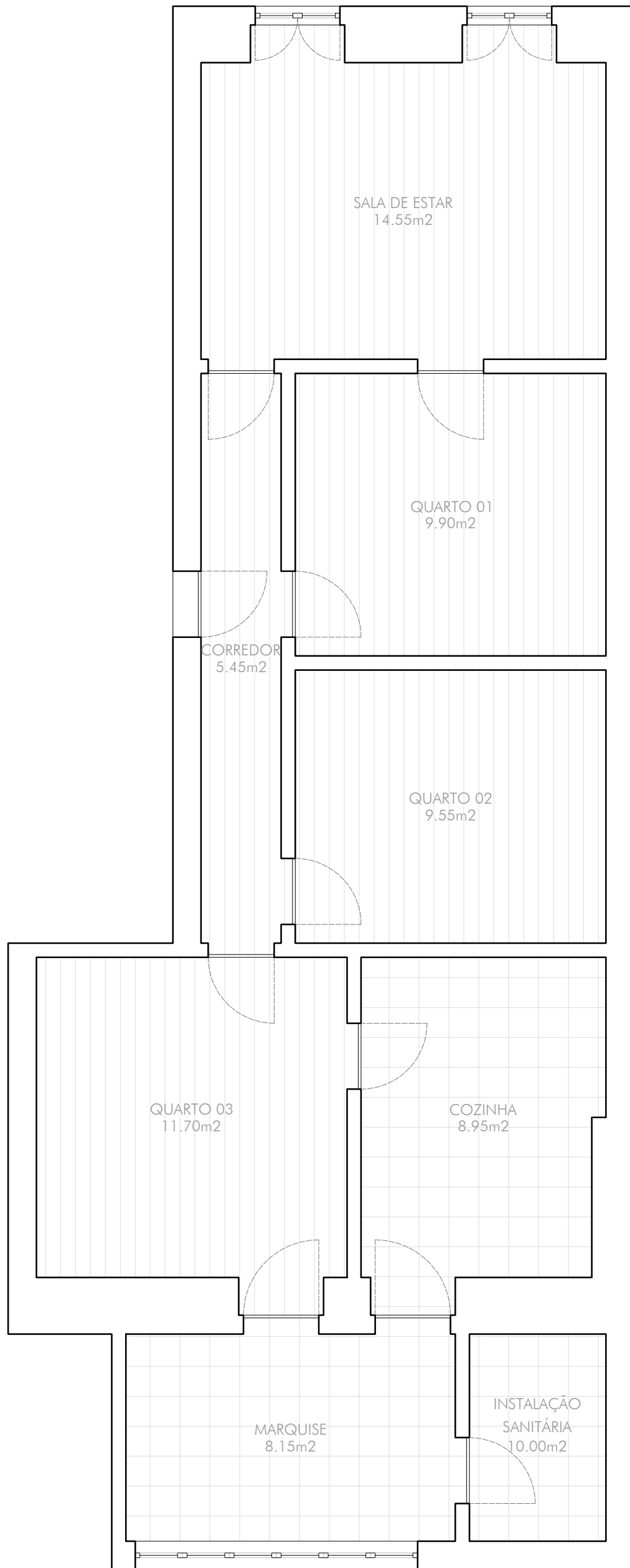
PLANTA DO EXISTENTE EXISTING FLOOR PLAN
